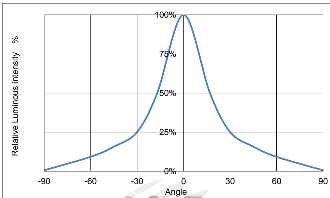
Fig 1-10 Radiation diagram
