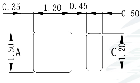
Fig.1-3 Bottom View
