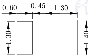
Fig.1-5 Soldering Patterns
