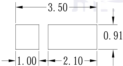
Fig 1-5 Soldering Patterns
