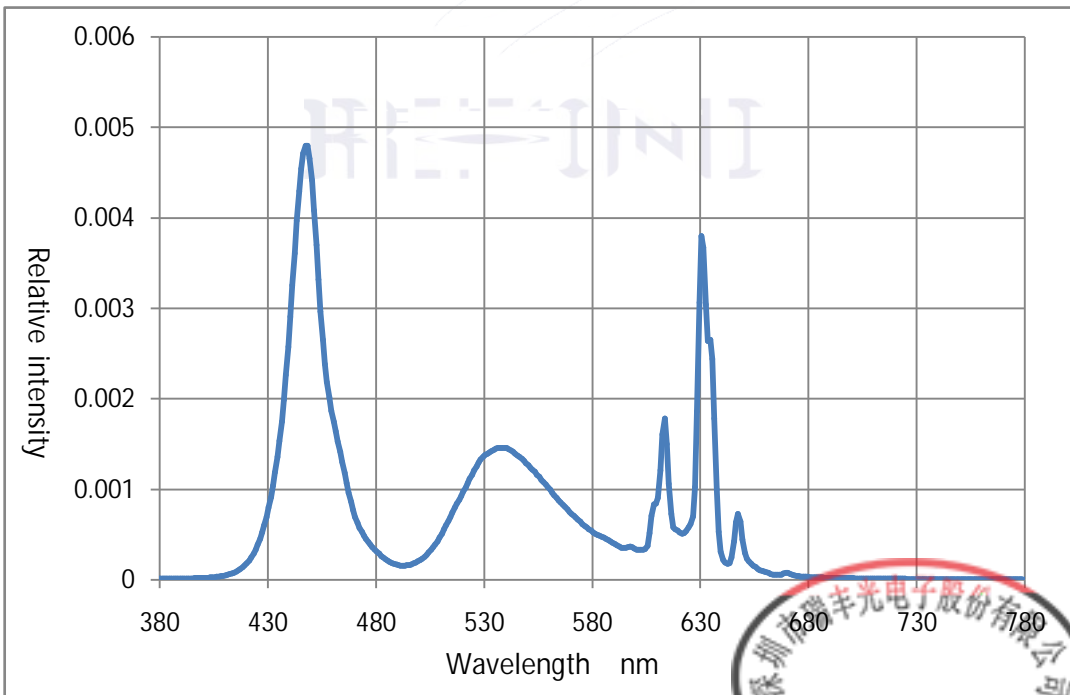
Fig. 1-14 Spectrum Distribution
