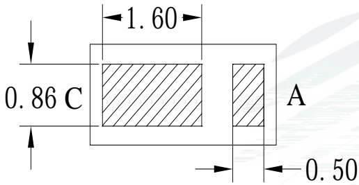
Fig 1-3 Bottom View
