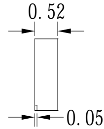
Fig 1-2 Side View
