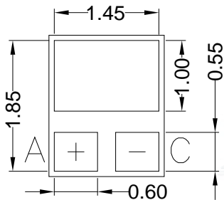
Fig.1-3 Bottom View
