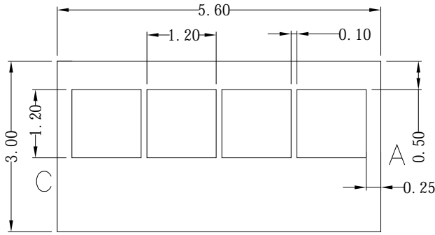
Fig.1-1 Top View
