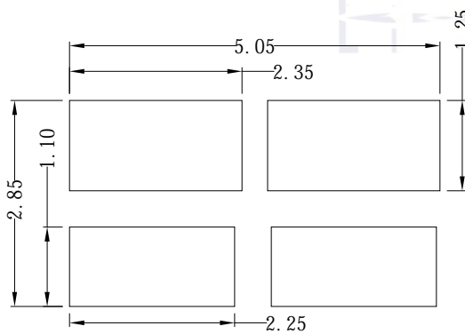
Fig.1-5 Soldering Patterns
