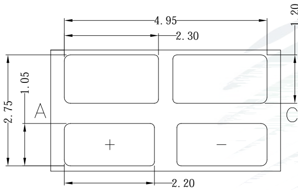
Fig.1-3 Bottom View
