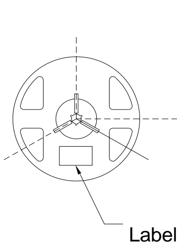
Fig.2-2 Reel 卷盘
