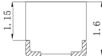
Fig.1-2 Side view 侧面视图
