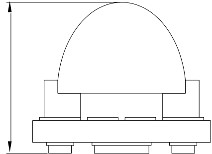
Fig.1-2 Side view
