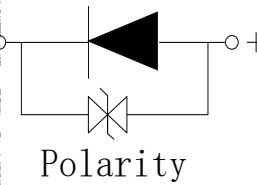
Fig.1-4 Polarity
