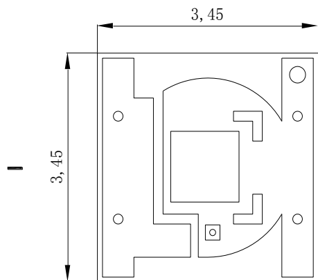
Fig.1-1 Top view
