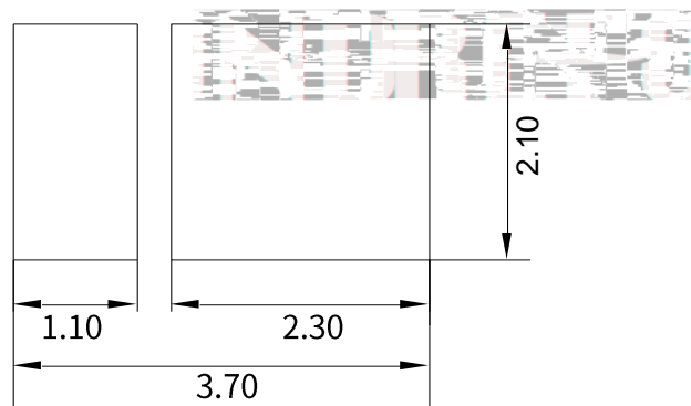
Fig.1-5 Soldering patterns 堆基焊盘
