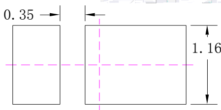
Fig.1-5 Soldering patterns
