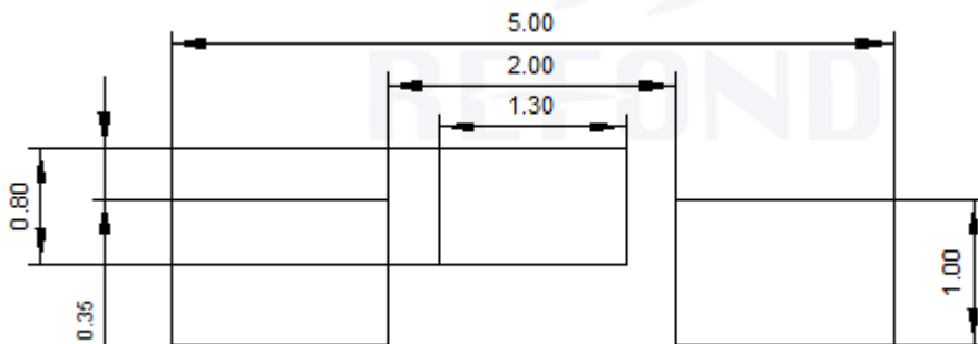
Fig.1-5 Soldering patterns
