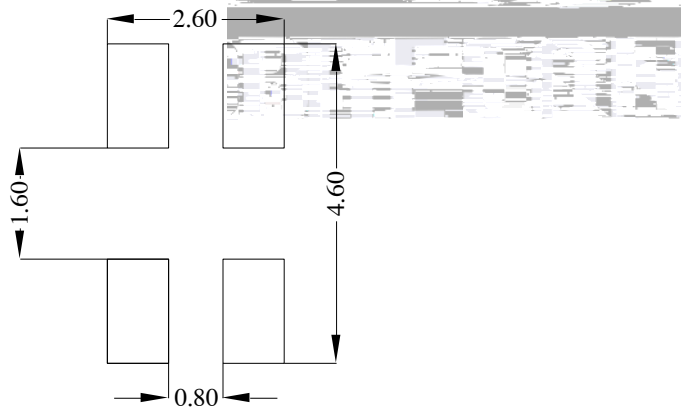
Fig.1-5 Soldering Patterns
